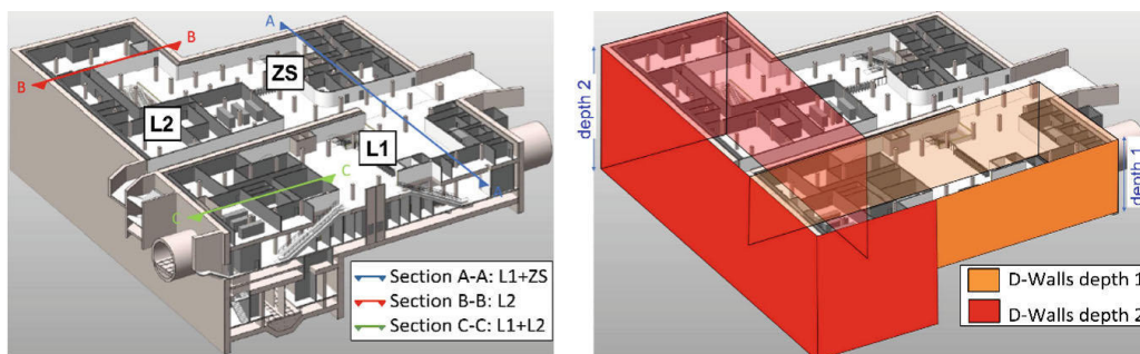
Fig. 3 Characteristic cross sections in the geotechnical analyses
