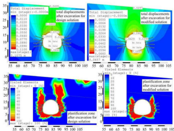
Figure 4. Stress-strain analyses for design and modified solution.
